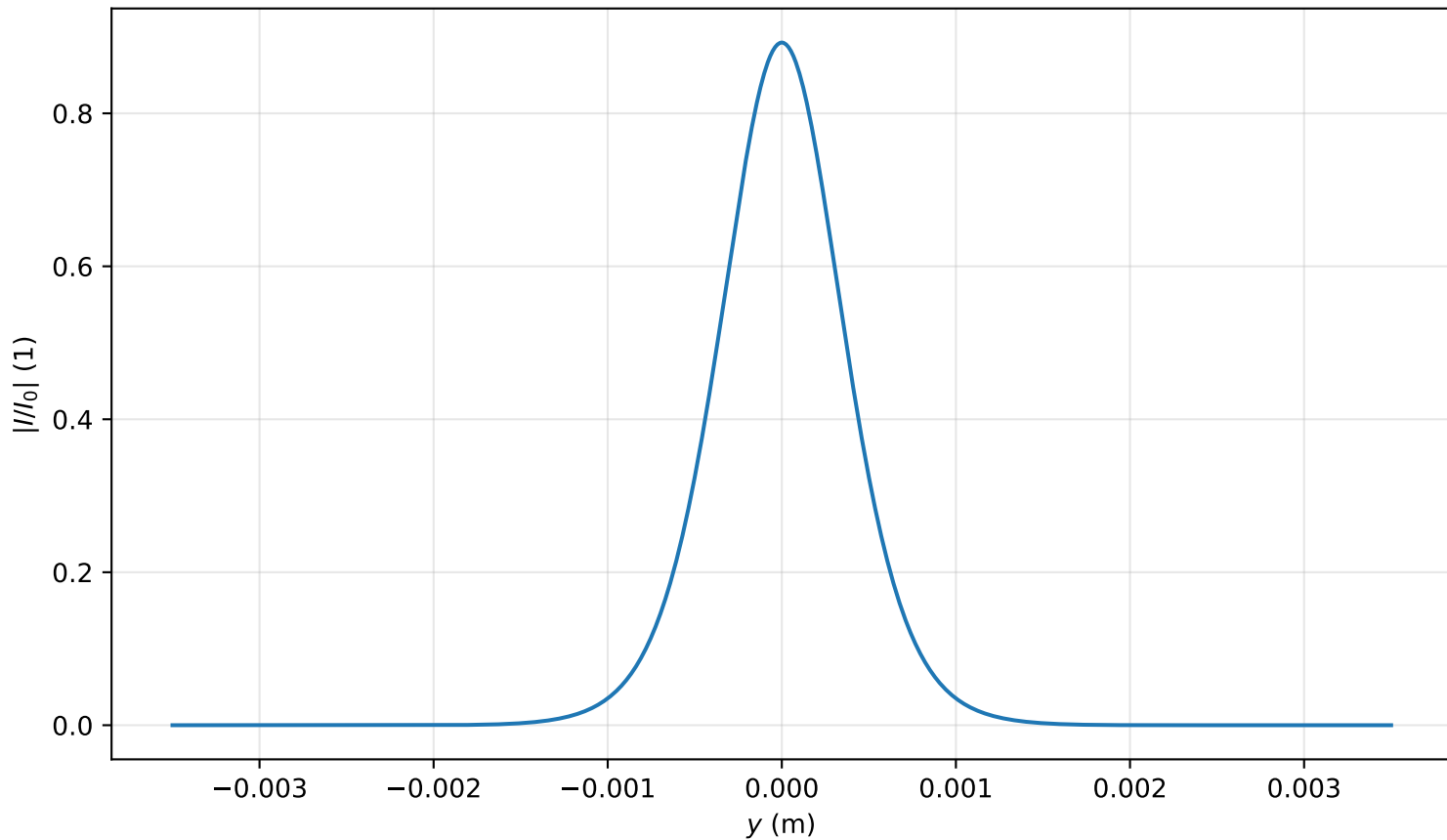
Intensity profile I(x=0, y, z=1.751)/I_0 , P_{in}=0.5P_{cr} , artificial time
